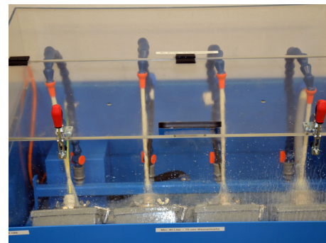
Oil Spray Test
