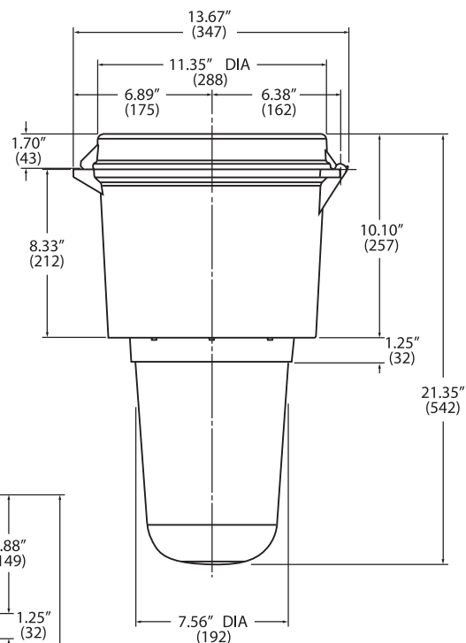
VM5 Fixture
