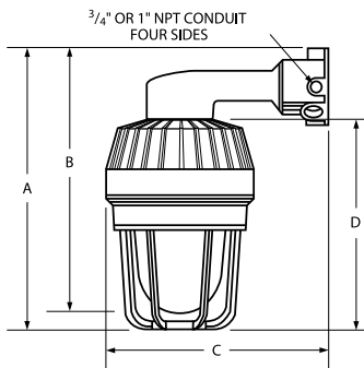
Wall
