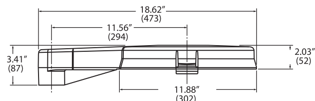
Stanchion(0°) Mount
