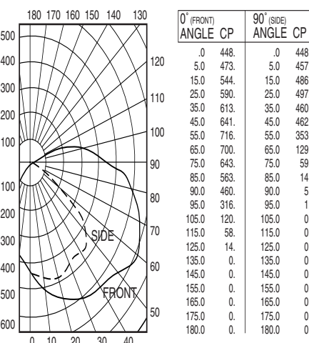
Coefficients of Utilization -- Zonal Cavity Method
