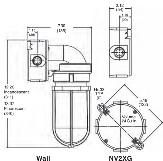
Wall
