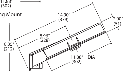
Stanchion(25°) Mount
