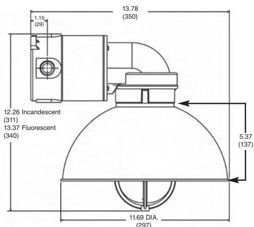
Wall
