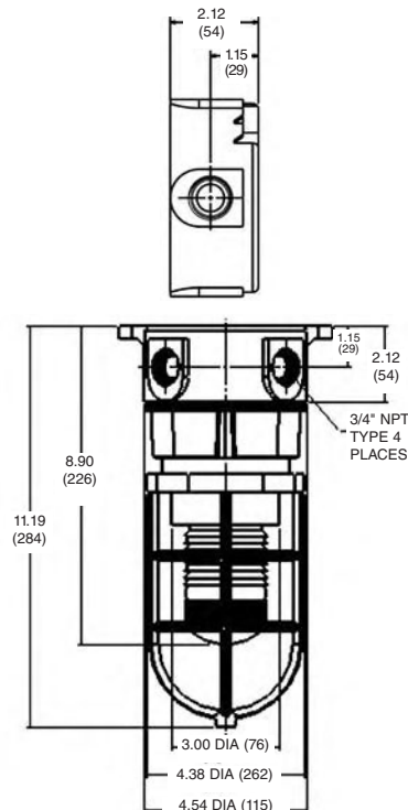
Ceiling/Wall NVSZ Xenon
