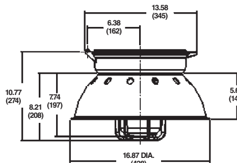
VM1L Tank with Dome Refractor
