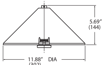
Cone Mount
