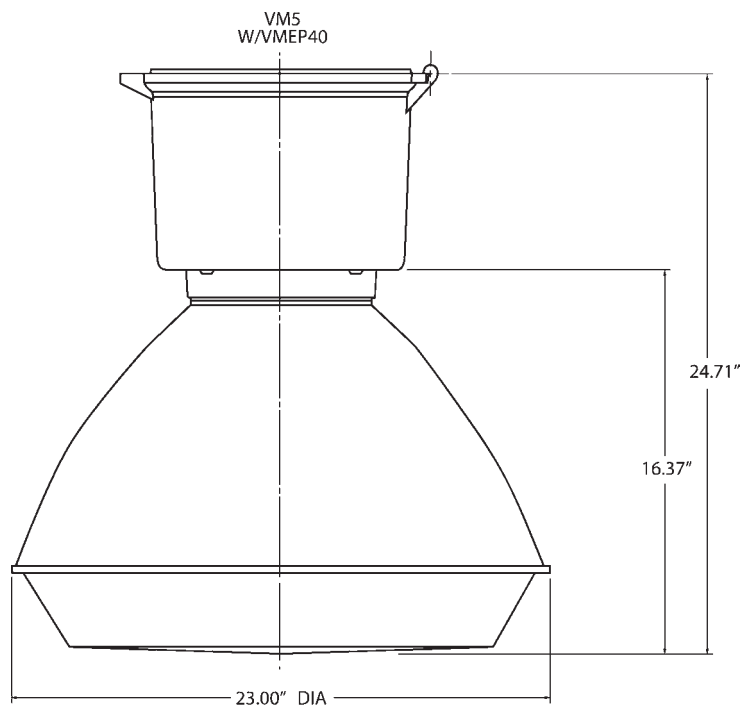
VM5 with VMEP40 Optic
