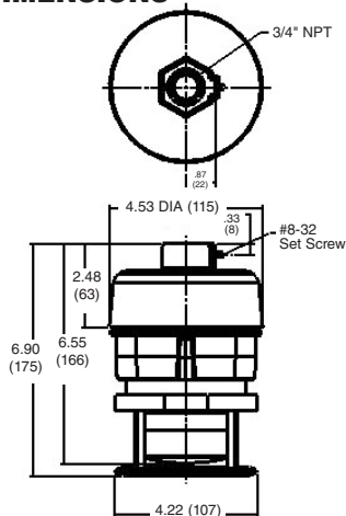
Pendant NVSL LED
