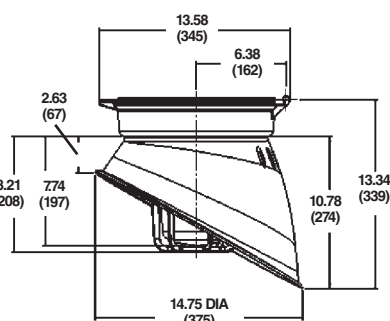
VM1L Tank with Angle Refractor
