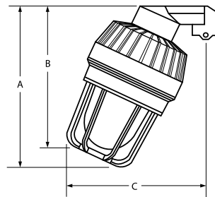
25° Stanchion
