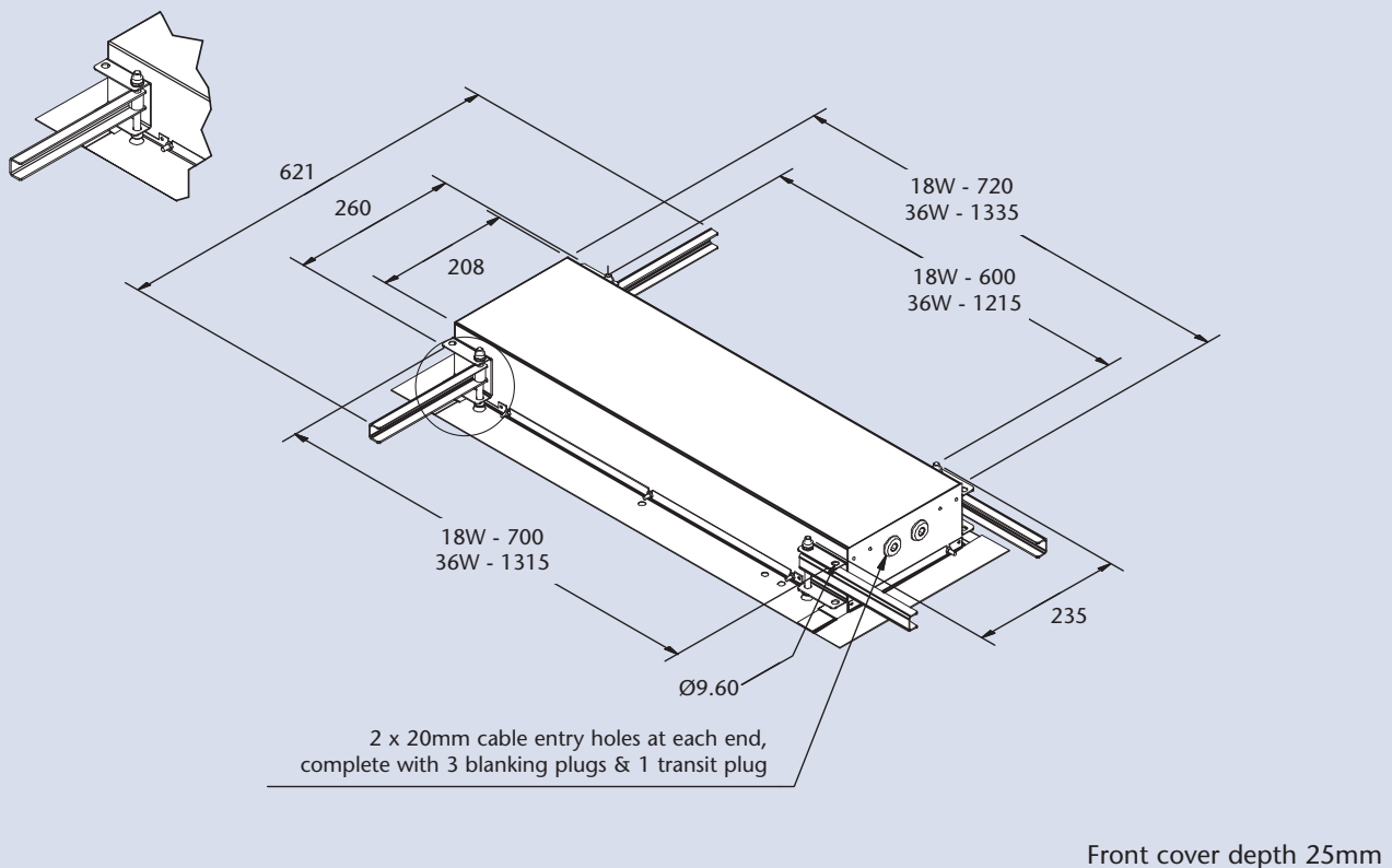
Rear view of recessed luminaire
