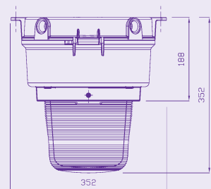
Prismatic glass refractor
