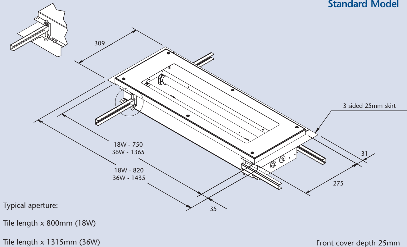
Front view of recessed luminaire
